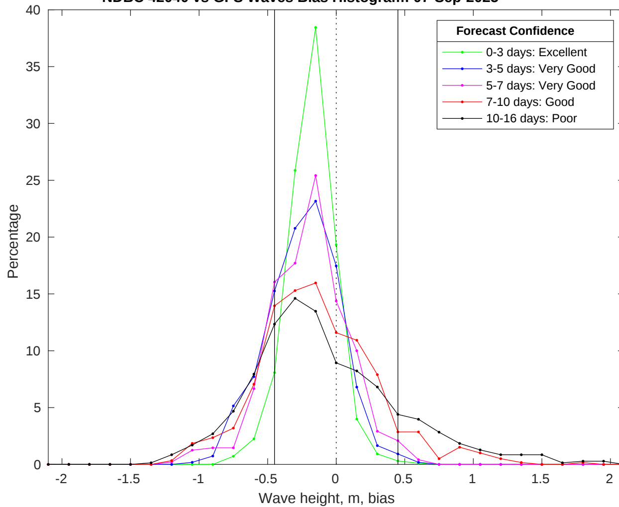
NDBC 42040 vs GFS Waves Bias Histogram: 07-Sep-2025
