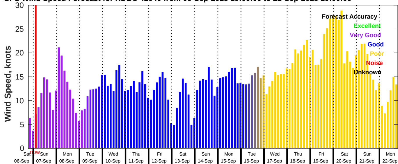
GFS Wind Speed Forecast for NDBC 42040 from 06-Sep-2025 19:00:00 to 22-Sep-2025 19:00:00
