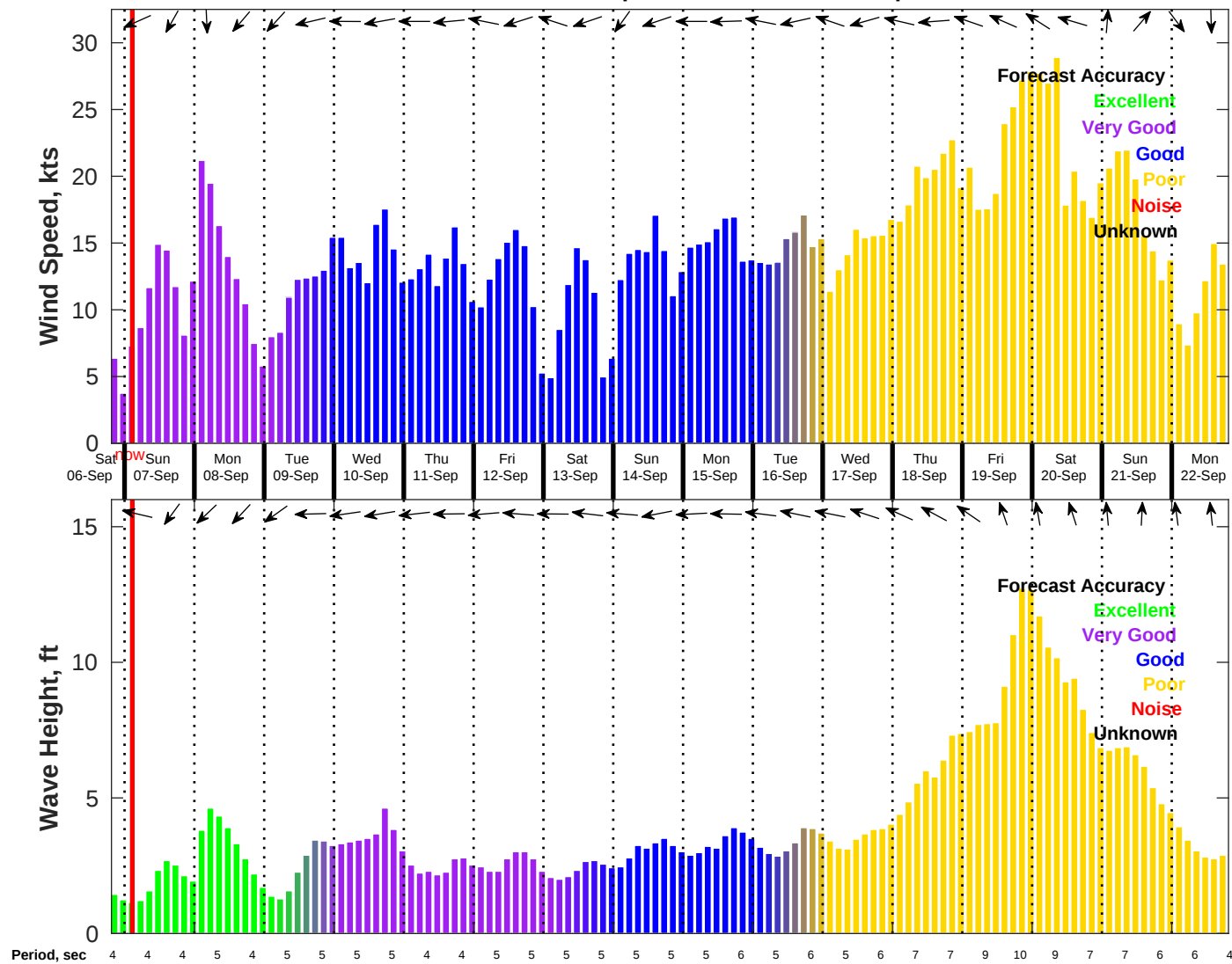
Wind & Wave Forecast for NDBC 42040 from 06-Sep-2025 19:00:00 to 22-Sep-2025 19:00:00
