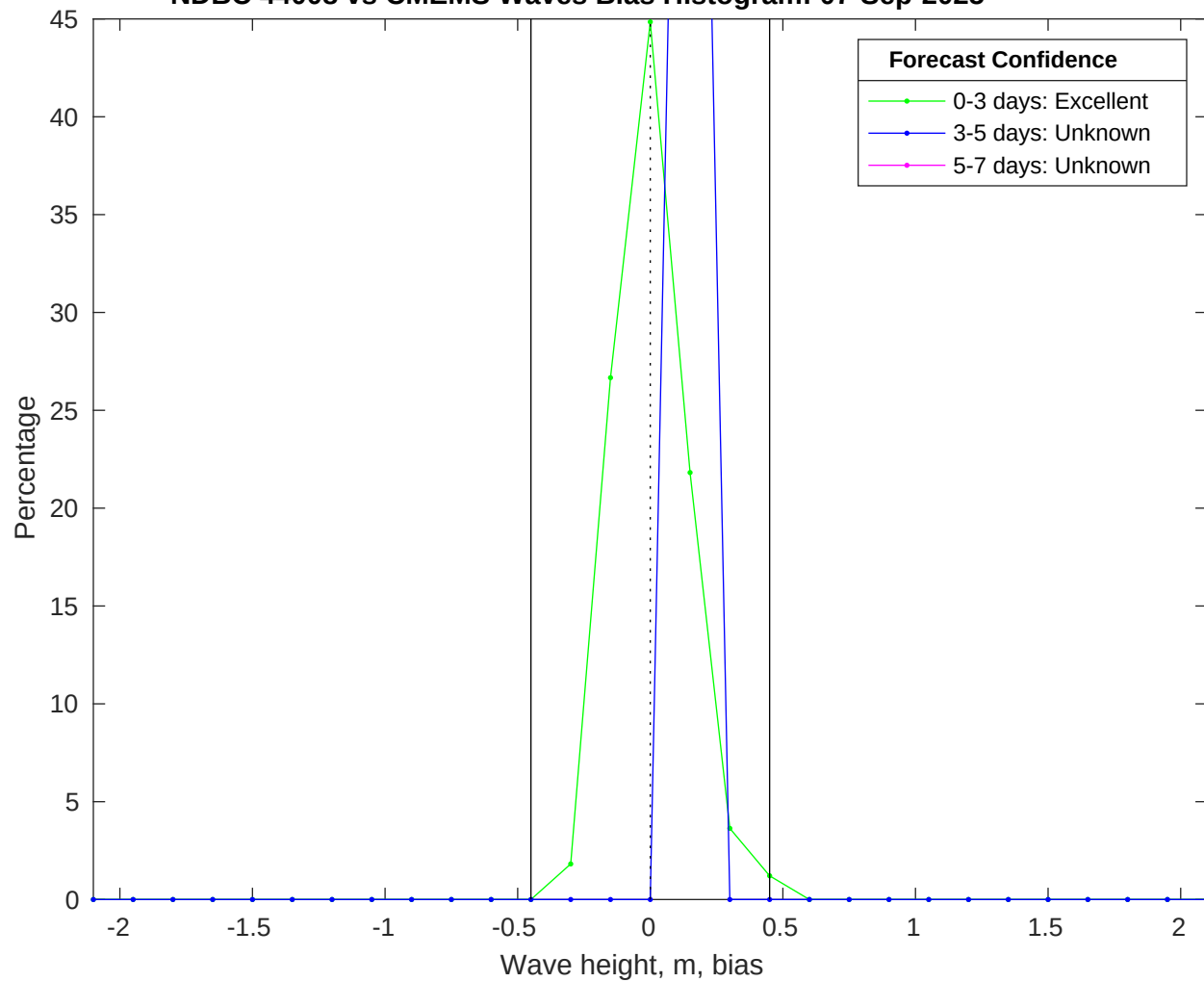
NDBC 44008 vs CMEMS Waves Bias Histogram: 07-Sep-2025
