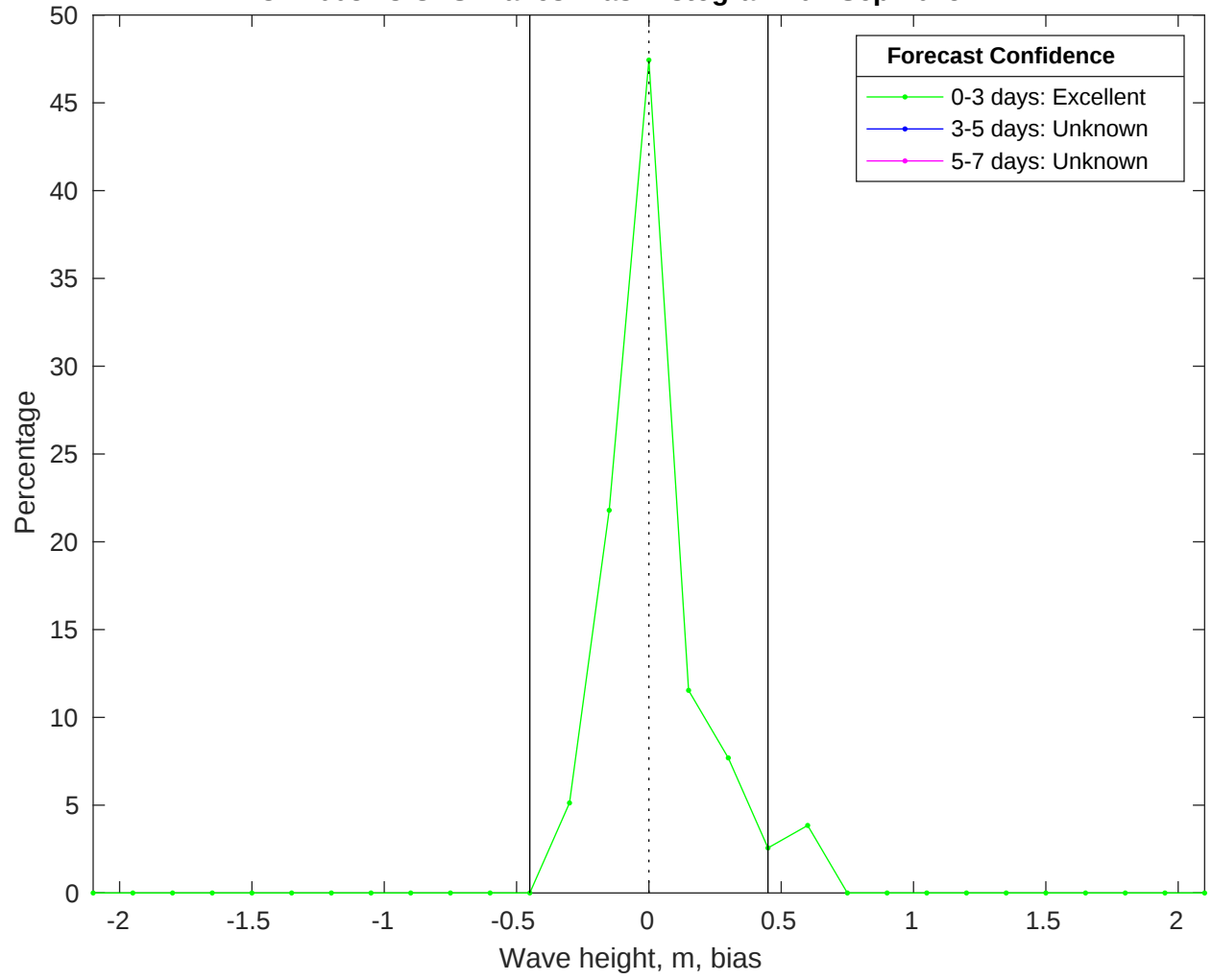
NDBC 44008 vs GFS Waves Bias Histogram: 07-Sep-2025
