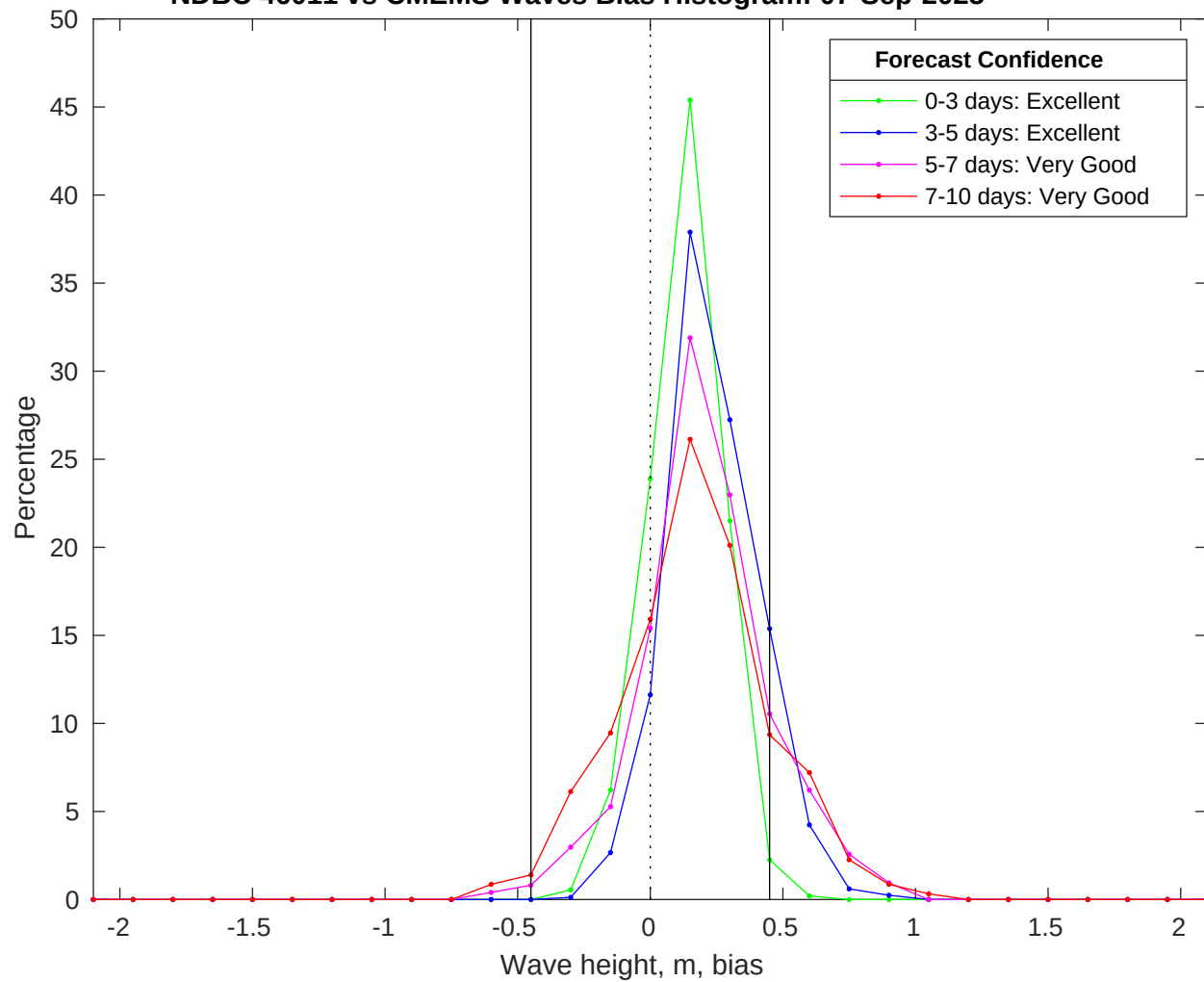
NDBC 46011 vs CMEMS Waves Bias Histogram: 07-Sep-2025
