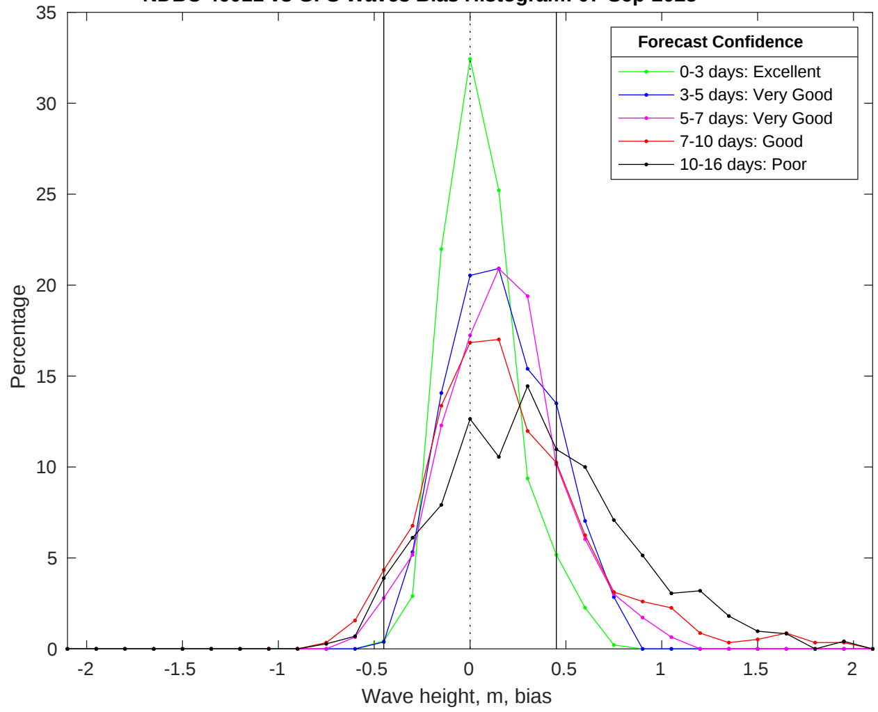
NDBC 46011 vs GFS Waves Bias Histogram: 07-Sep-2025
