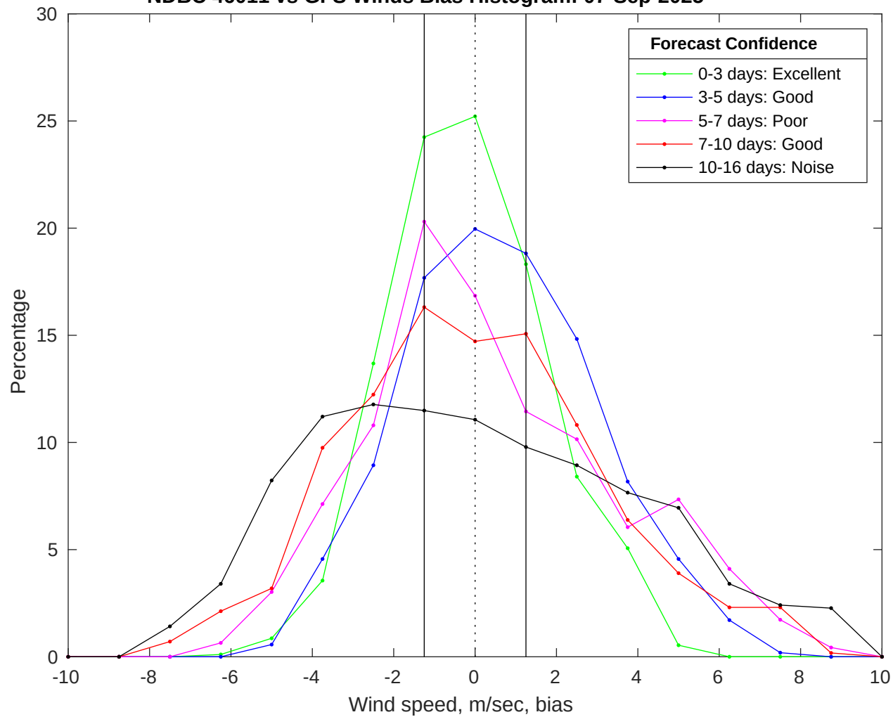
NDBC 46011 vs GFS Winds Bias Histogram: 07-Sep-2025
