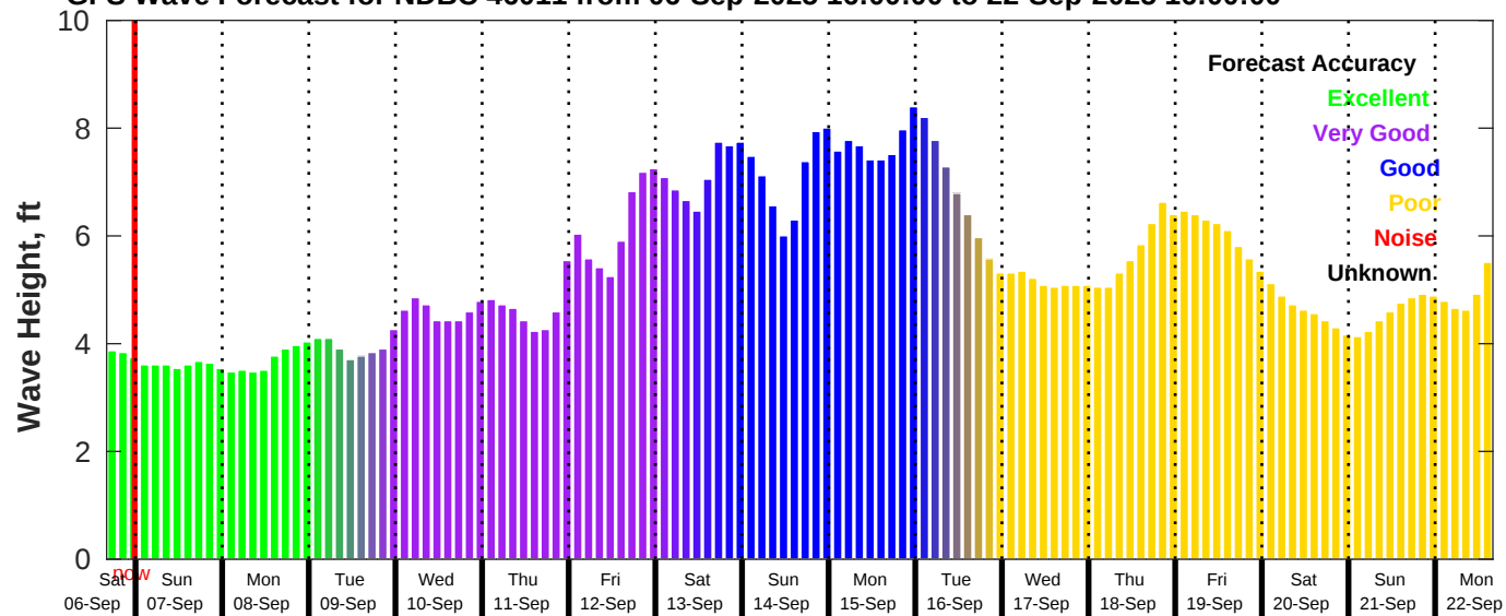
GFS Wave Forecast for NDBC 46011 from 06-Sep-2025 16:00:00 to 22-Sep-2025 16:00:00
