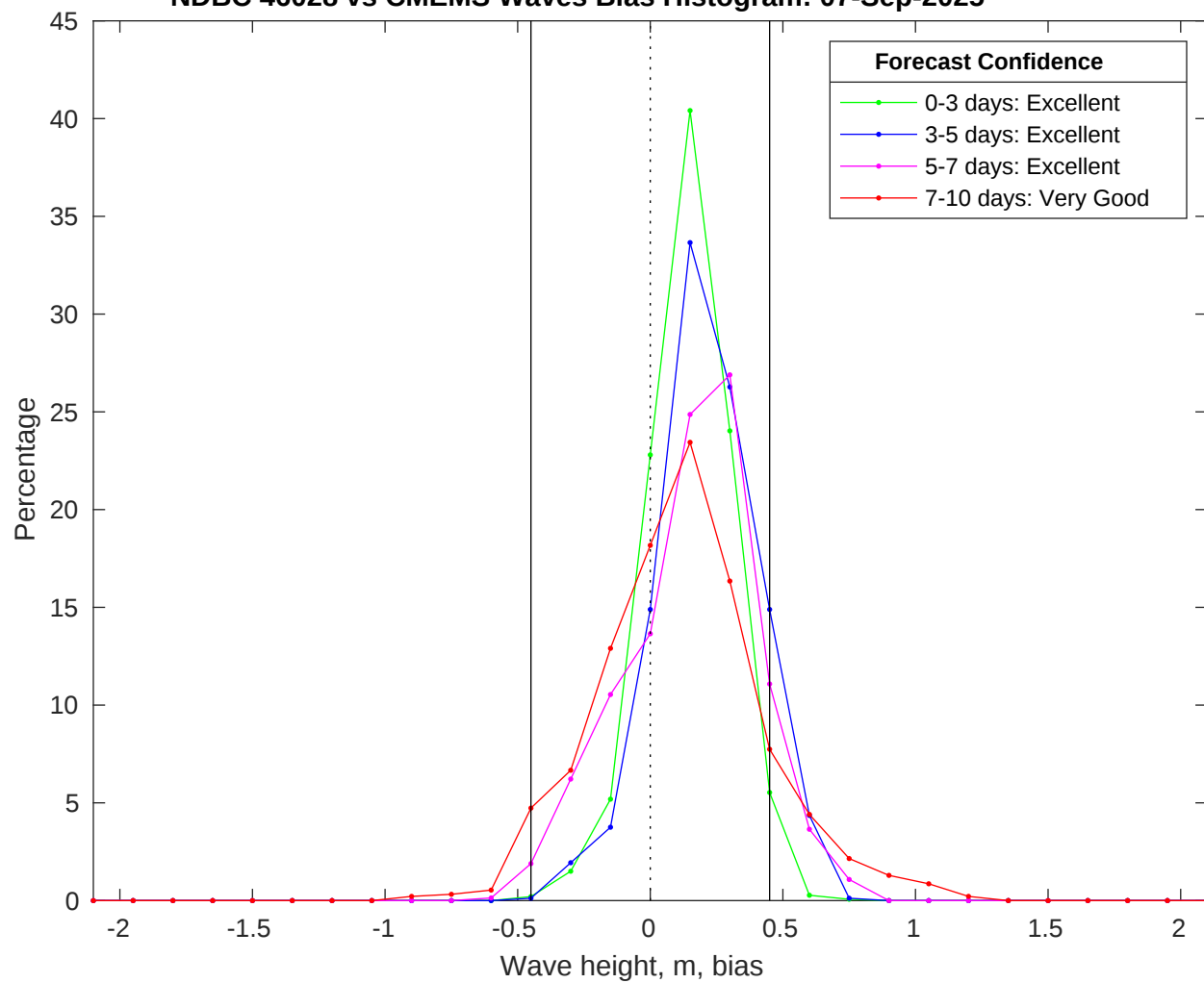
NDBC 46028 vs CMEMS Waves Bias Histogram: 07-Sep-2025
