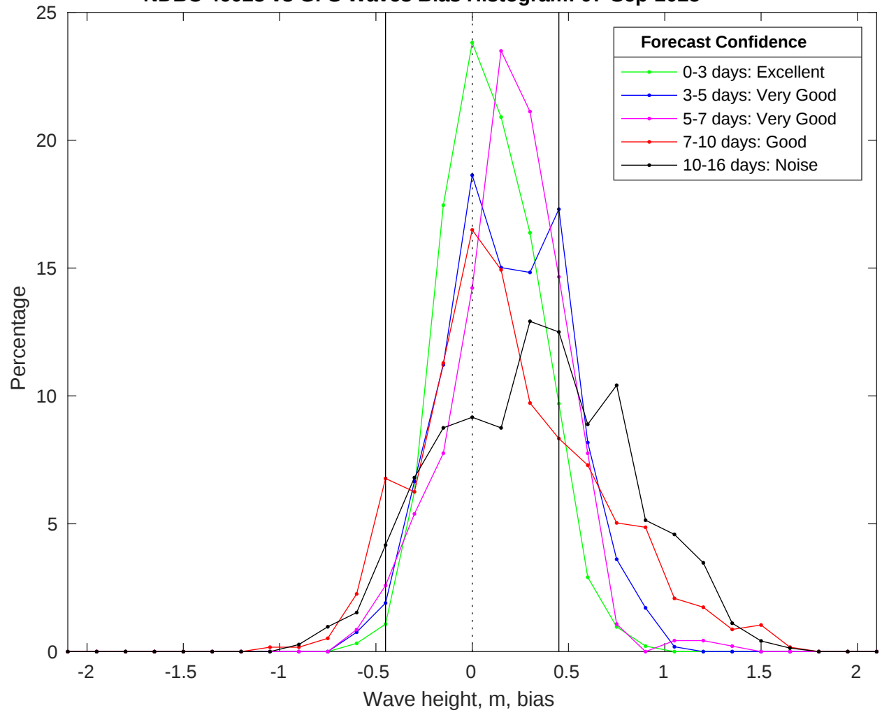
NDBC 46028 vs GFS Waves Bias Histogram: 07-Sep-2025
