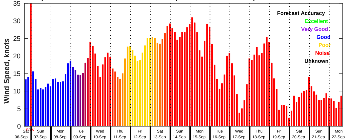
GFS Wind Speed Forecast for NDBC 46028 from 06-Sep-2025 16:00:00 to 22-Sep-2025 16:00:00
