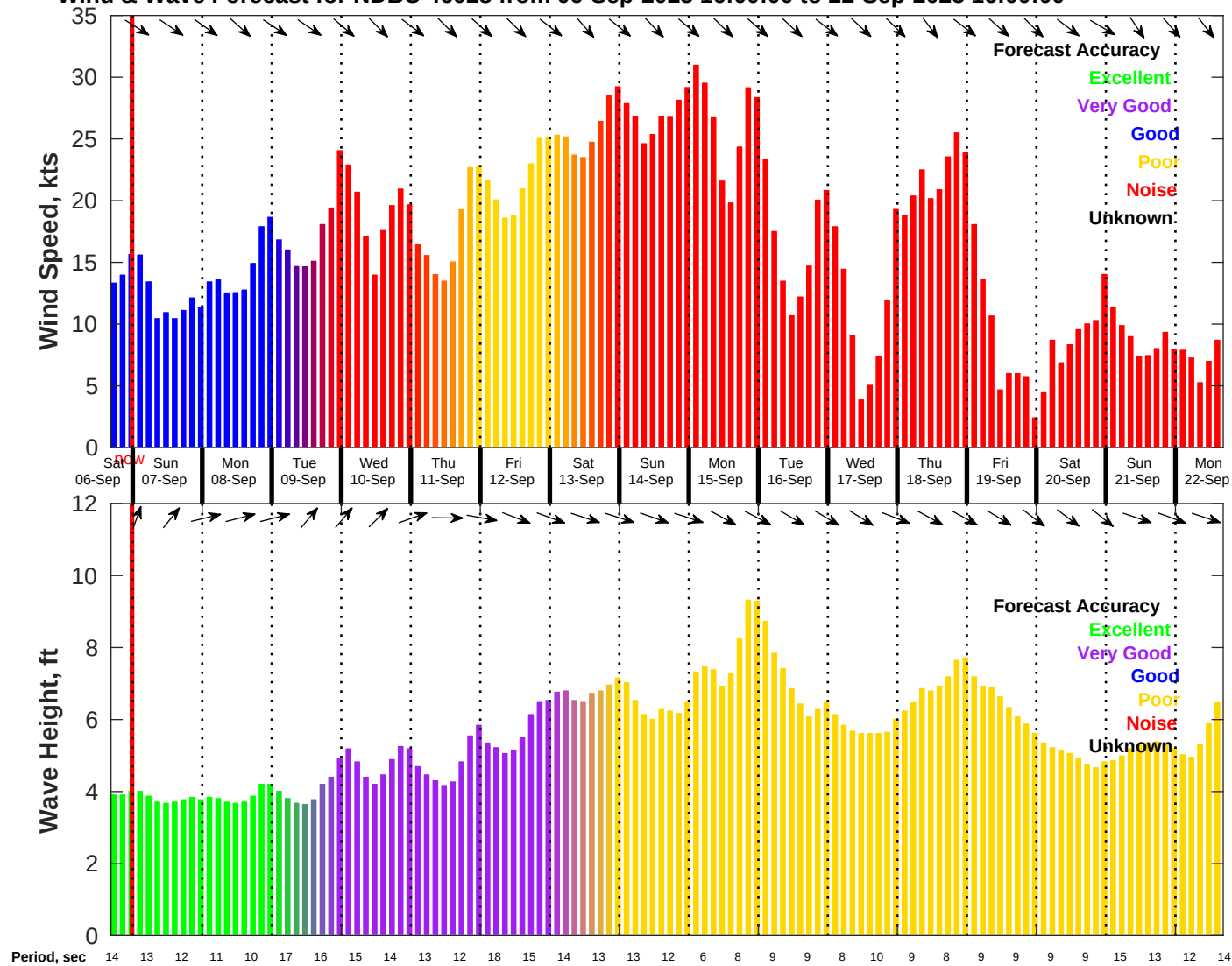
Wind & Wave Forecast for NDBC 46028 from 06-Sep-2025 16:00:00 to 22-Sep-2025 16:00:00
