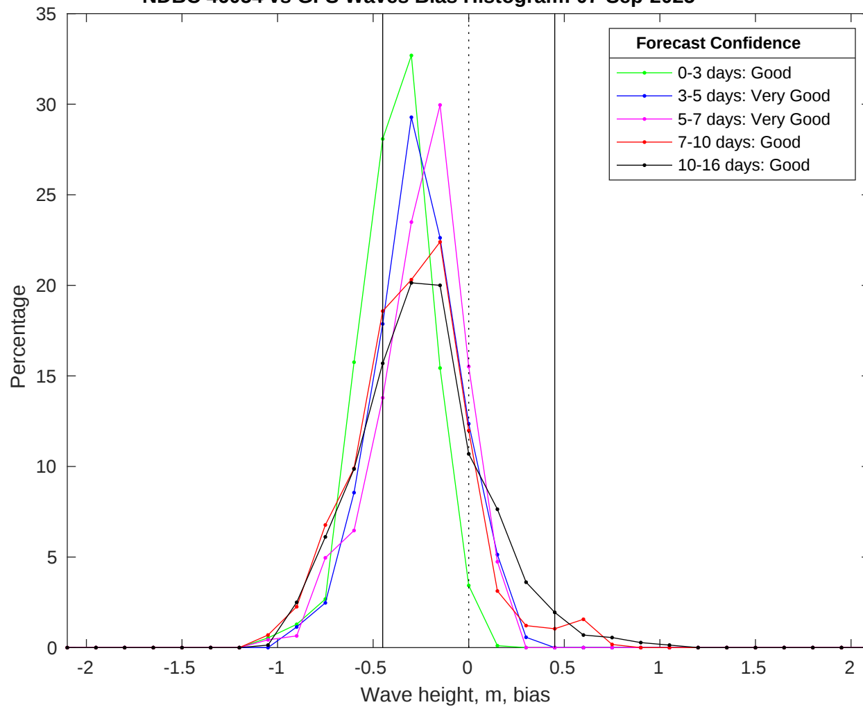
NDBC 46054 vs GFS Waves Bias Histogram: 07-Sep-2025
