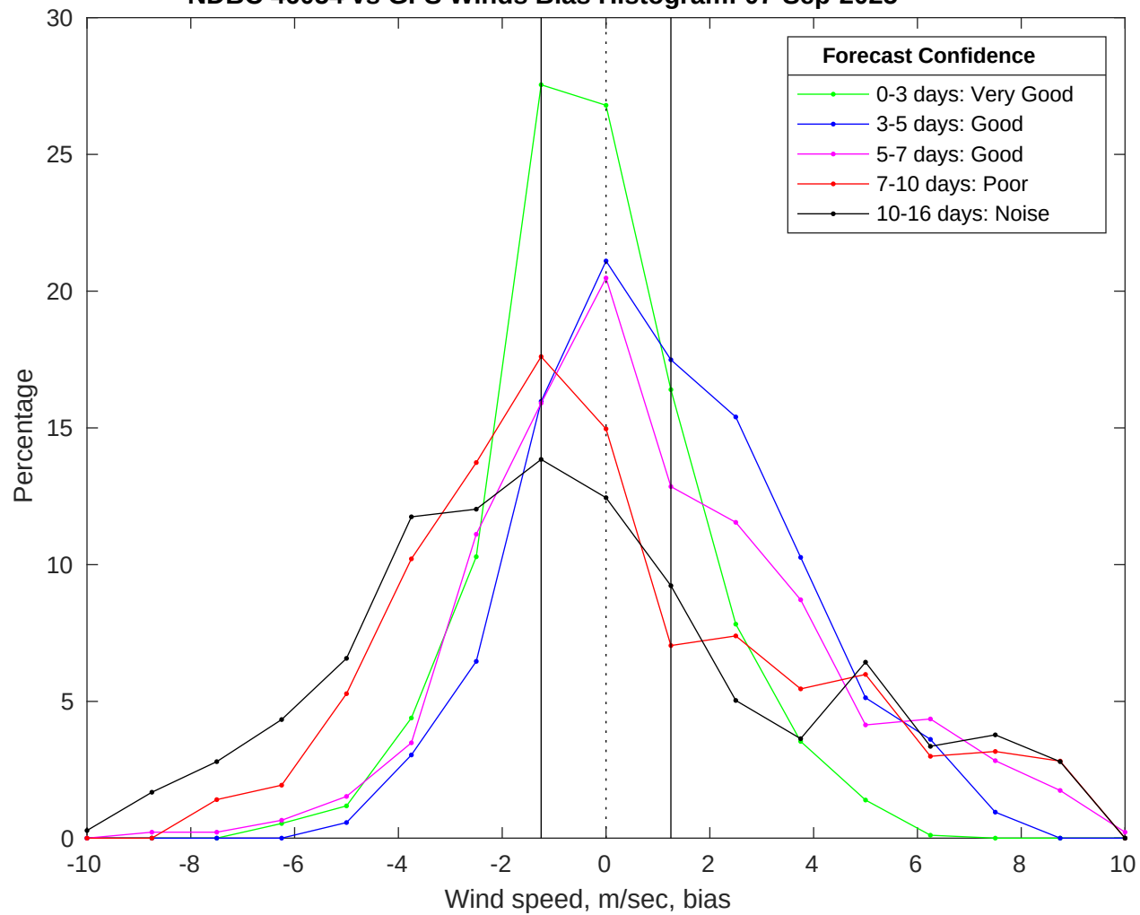
NDBC 46054 vs GFS Winds Bias Histogram: 07-Sep-2025
