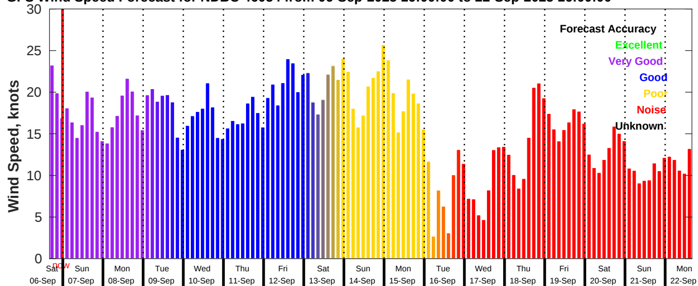
GFS Wind Speed Forecast for NDBC 46054 from 06-Sep-2025 16:00:00 to 22-Sep-2025 16:00:00
