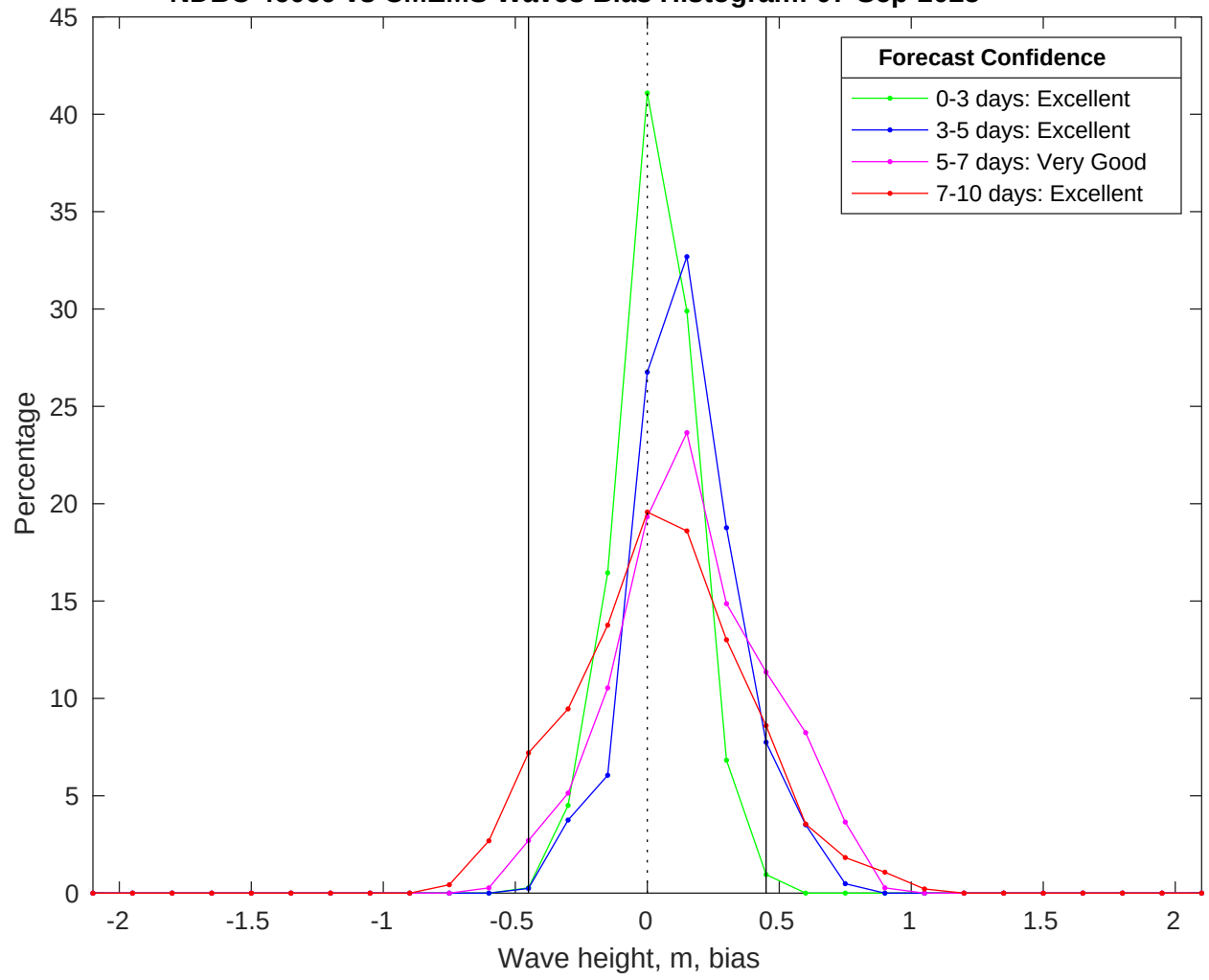
NDBC 46069 vs CMEMS Waves Bias Histogram: 07-Sep-2025
