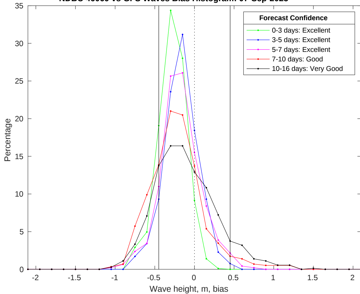
NDBC 46069 vs GFS Waves Bias Histogram: 07-Sep-2025
