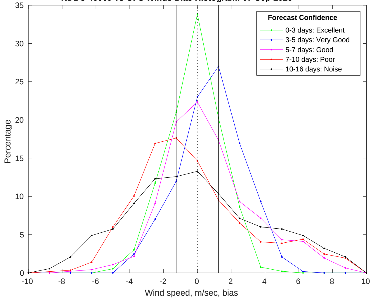
NDBC 46069 vs GFS Winds Bias Histogram: 07-Sep-2025
