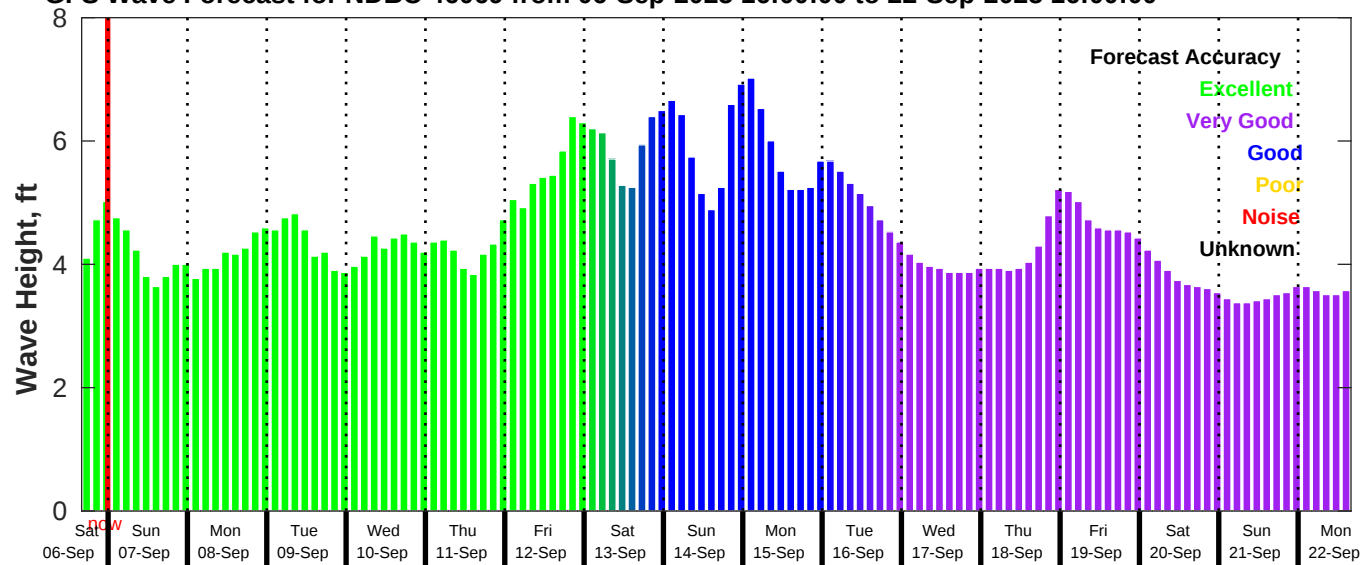
GFS Wave Forecast for NDBC 46069 from 06-Sep-2025 16:00:00 to 22-Sep-2025 16:00:00
