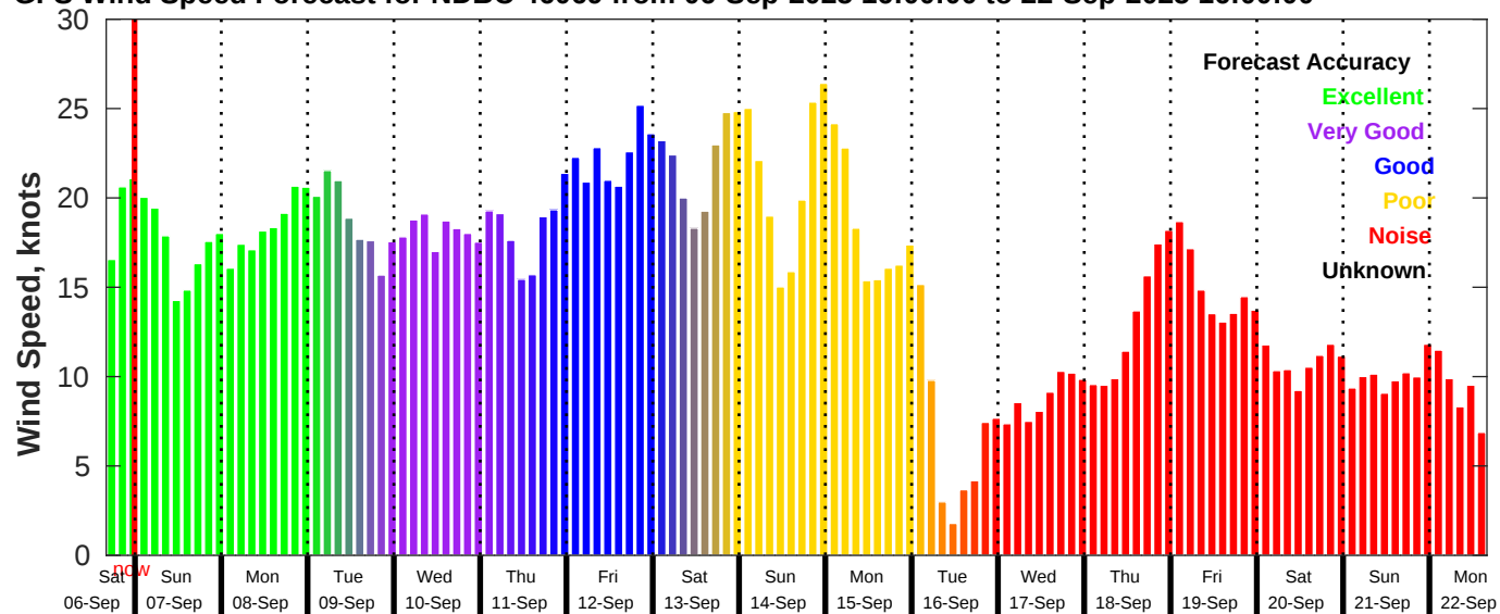
GFS Wind Speed Forecast for NDBC 46069 from 06-Sep-2025 16:00:00 to 22-Sep-2025 16:00:00
