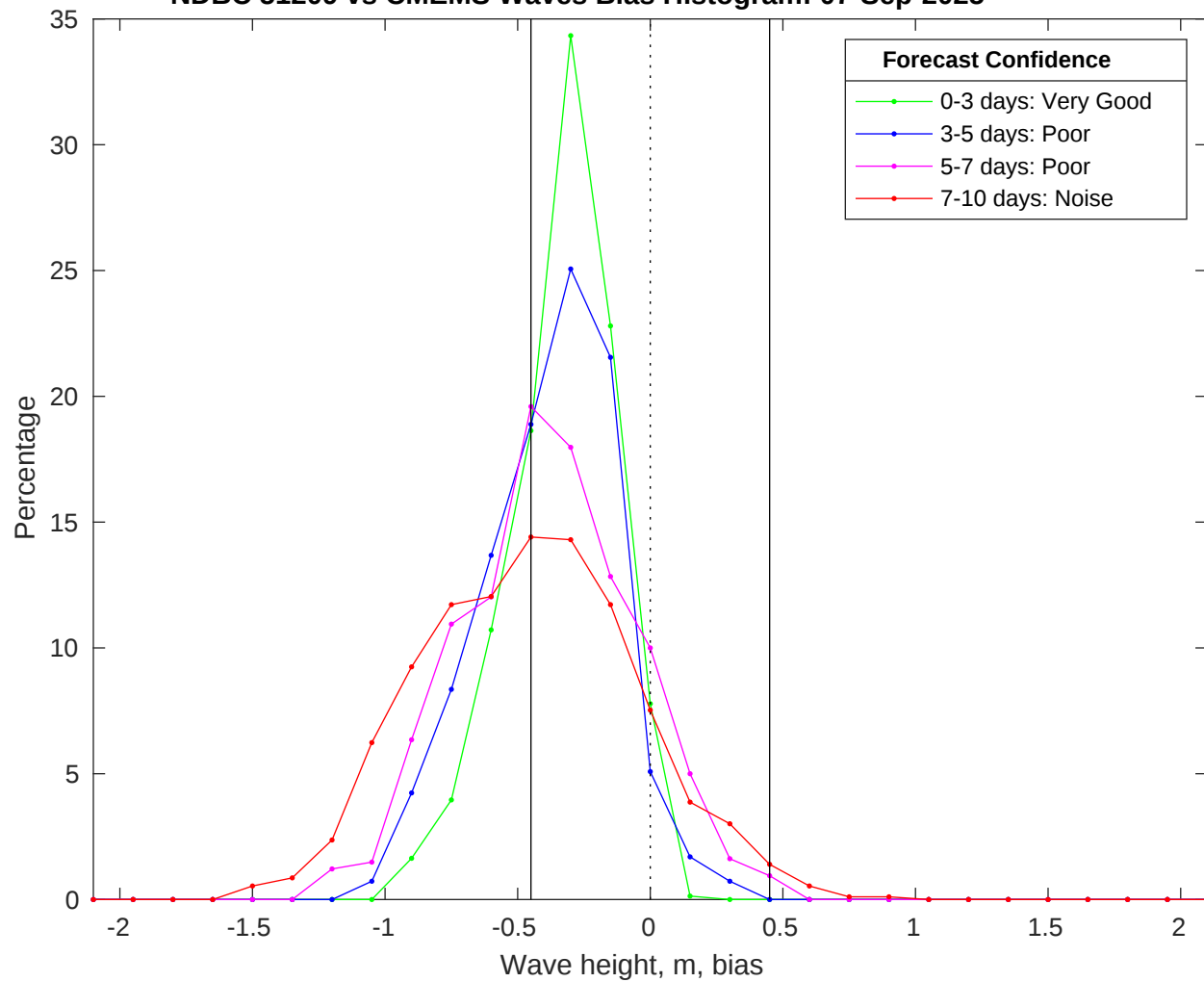
NDBC 51209 vs CMEMS Waves Bias Histogram: 07-Sep-2025
