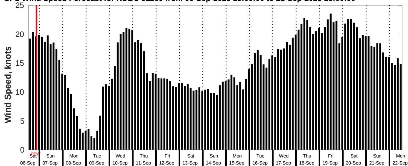
GFS Wind Speed Forecast for NDBC 51209 from 06-Sep-2025 13:00:00 to 22-Sep-2025 13:00:00
