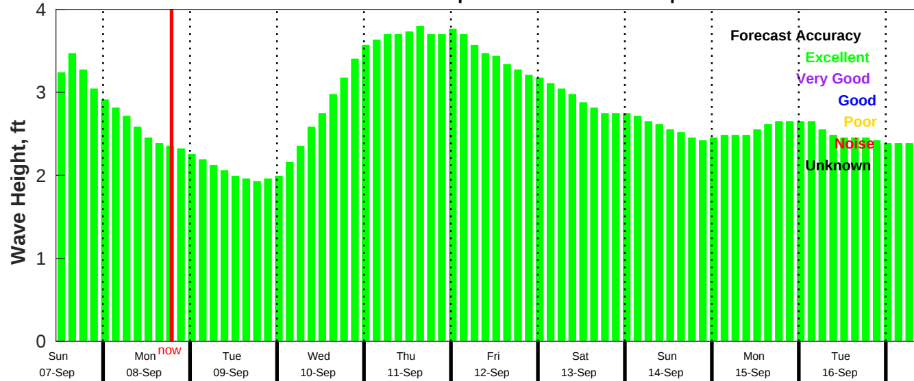
CMEMS Wave Forecast for NDBC 52211 from 06-Sep-2025 11:00:00 to 16-Sep-2025 11:00:00
