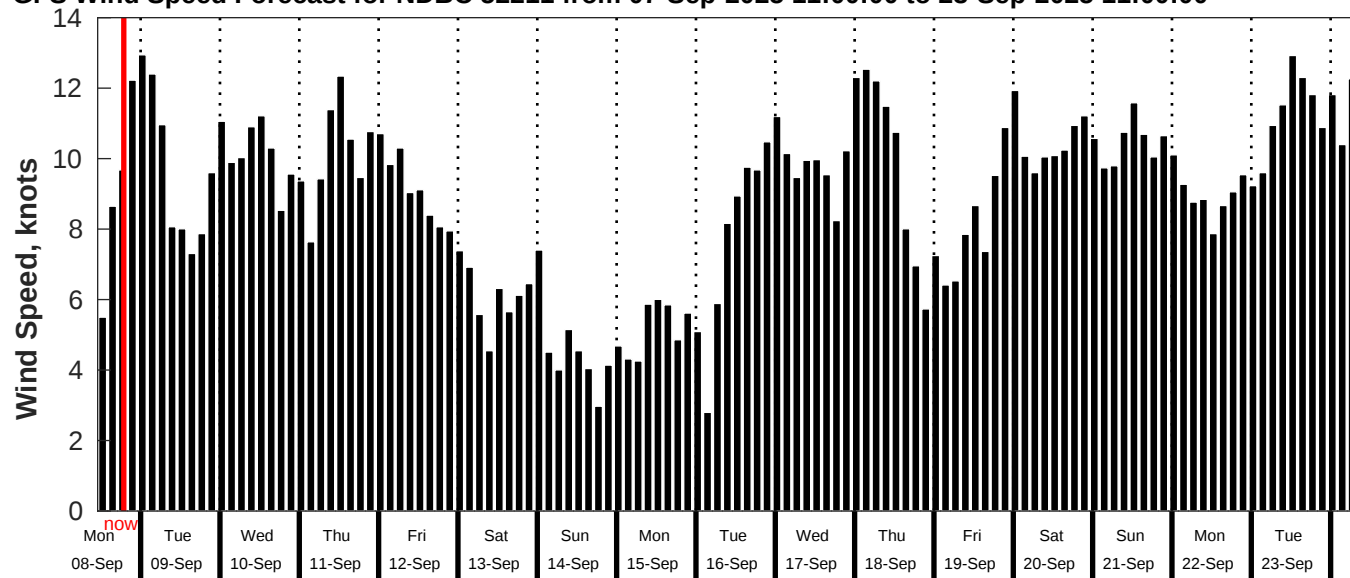
GFS Wind Speed Forecast for NDBC 52211 from 07-Sep-2025 11:00:00 to 23-Sep-2025 11:00:00
