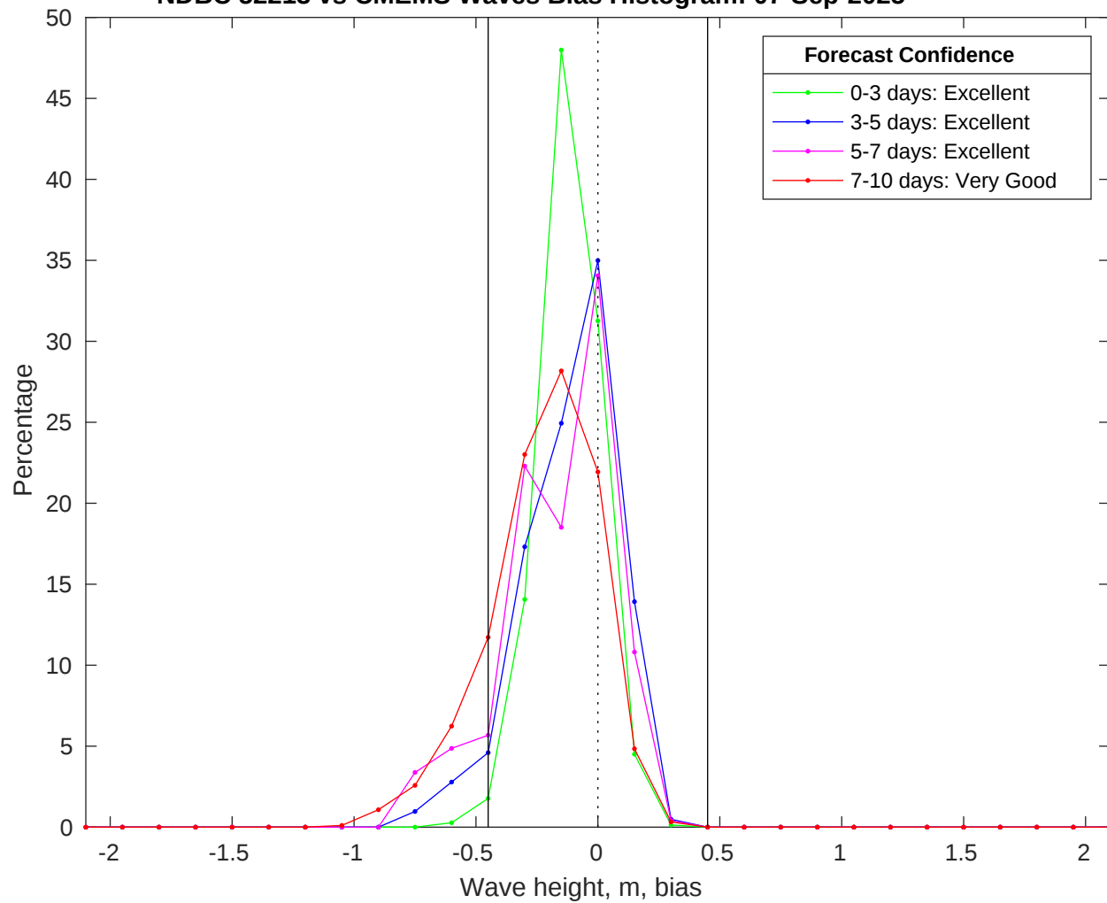
NDBC 52213 vs CMEMS Waves Bias Histogram: 07-Sep-2025
