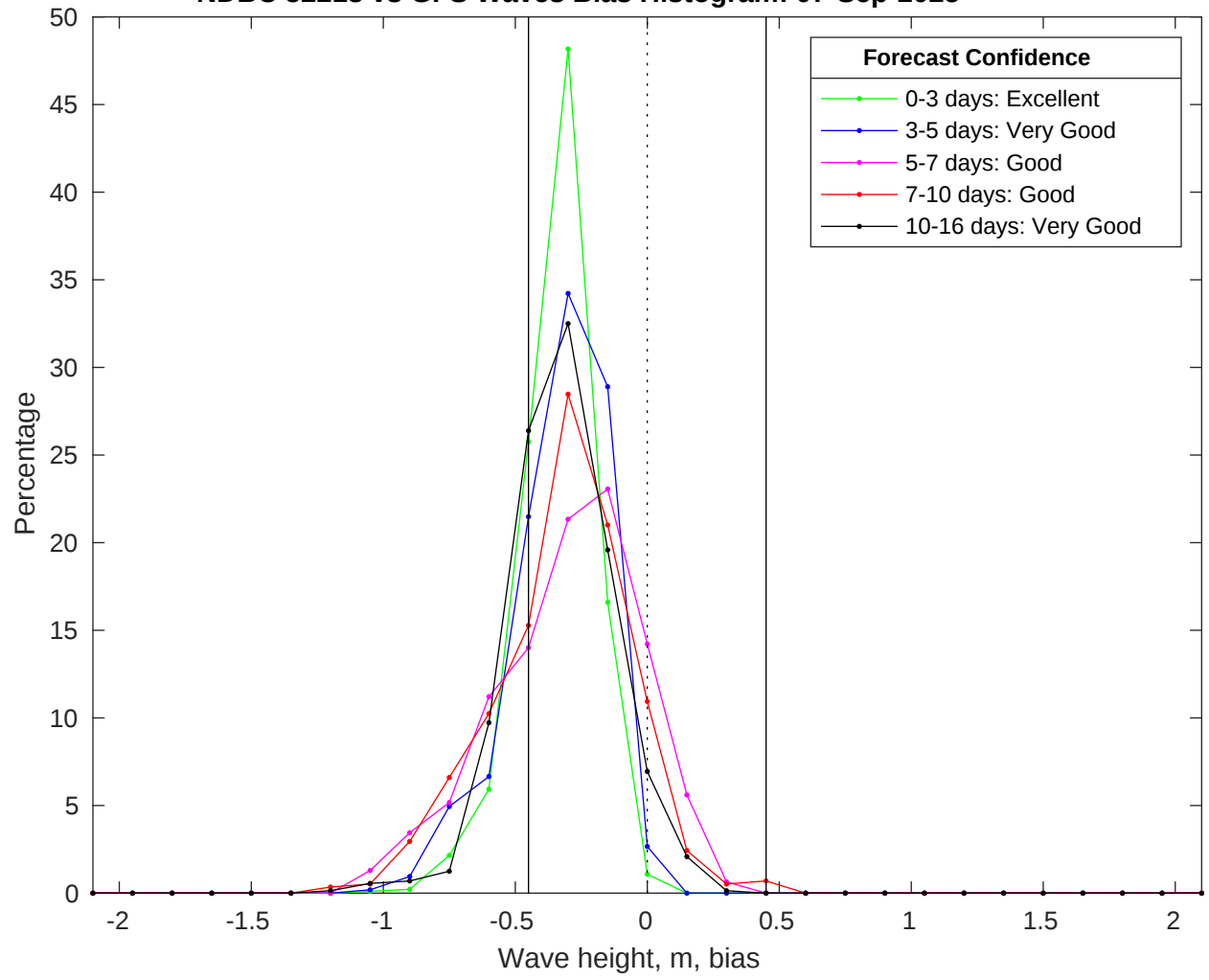
NDBC 52213 vs GFS Waves Bias Histogram: 07-Sep-2025
