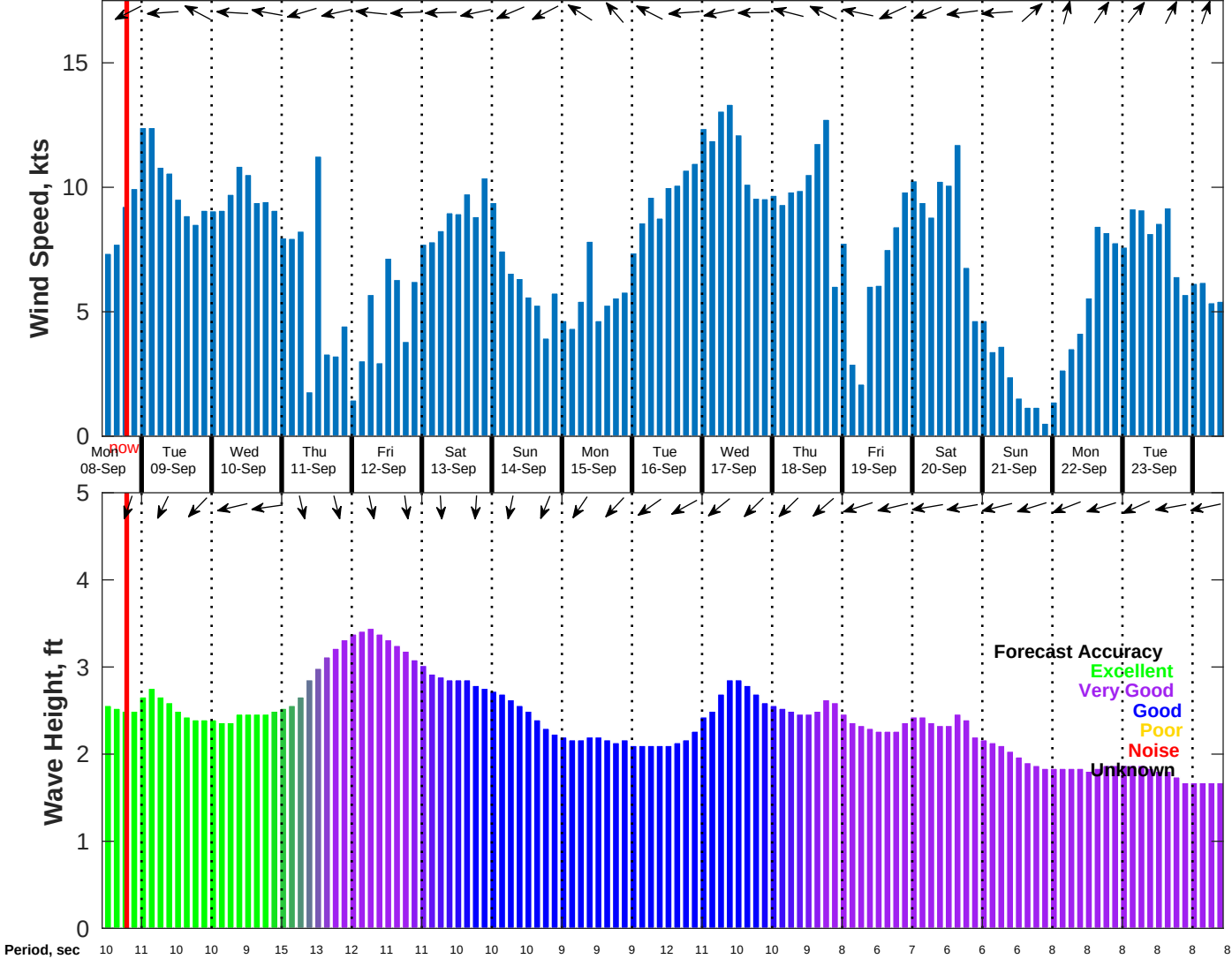
Wind & Wave Forecast for NDBC 52213 from 07-Sep-2025 11:00:00 to 23-Sep-2025 11:00:00
