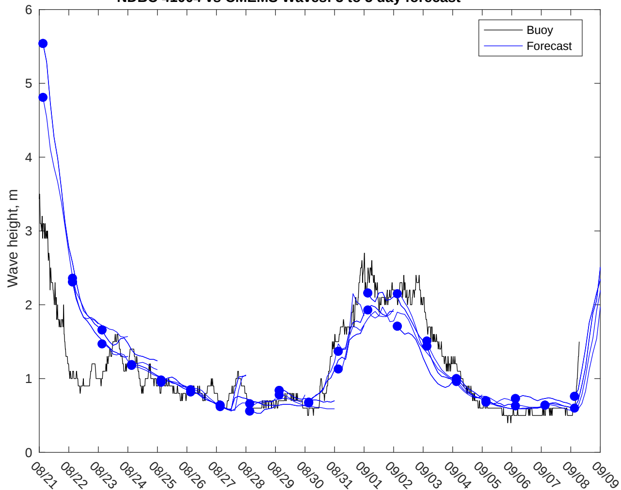
NDBC 41004 vs CMEMS Waves: 3 to 5 day forecast
