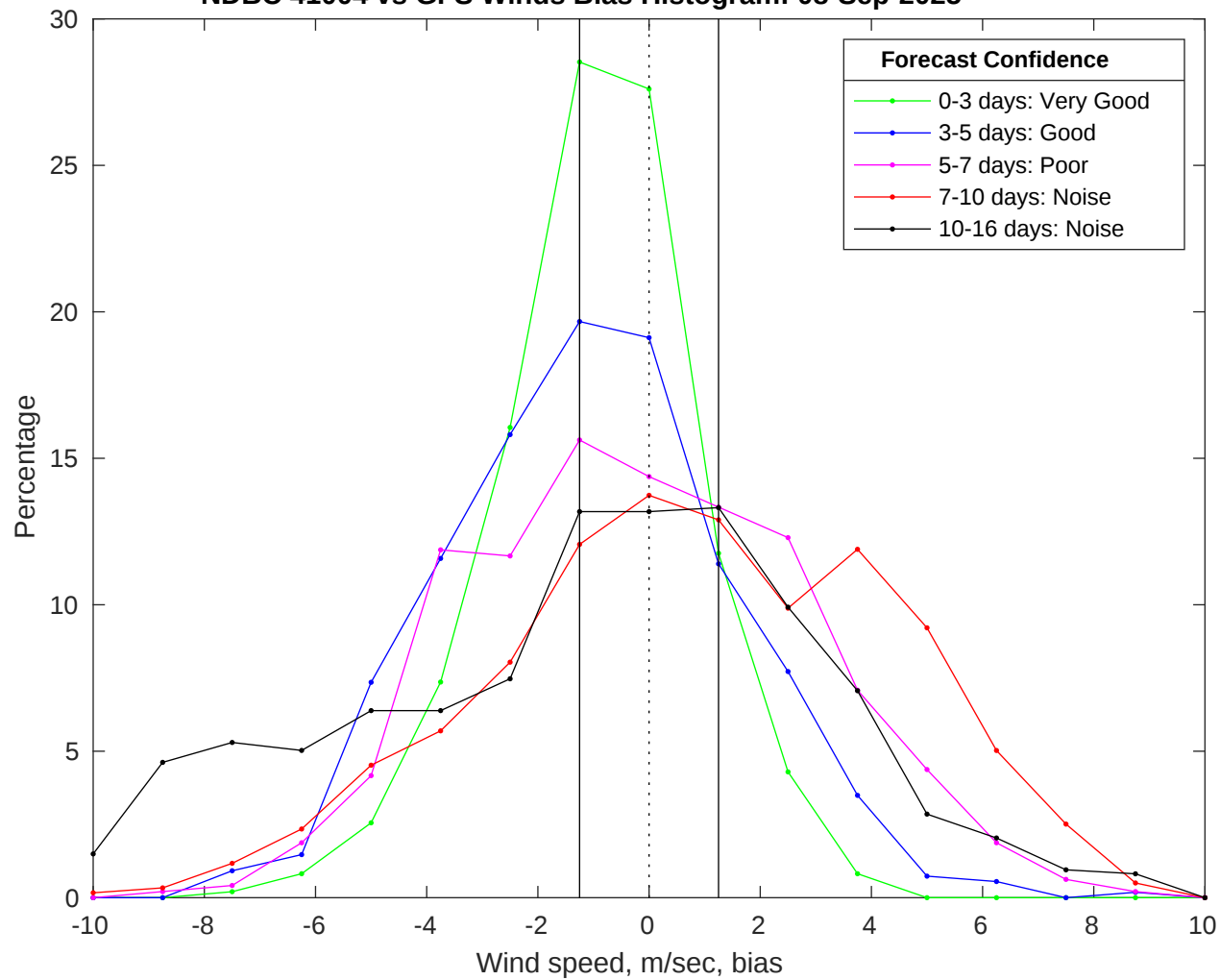
NDBC 41004 vs GFS Winds Bias Histogram: 08-Sep-2025
