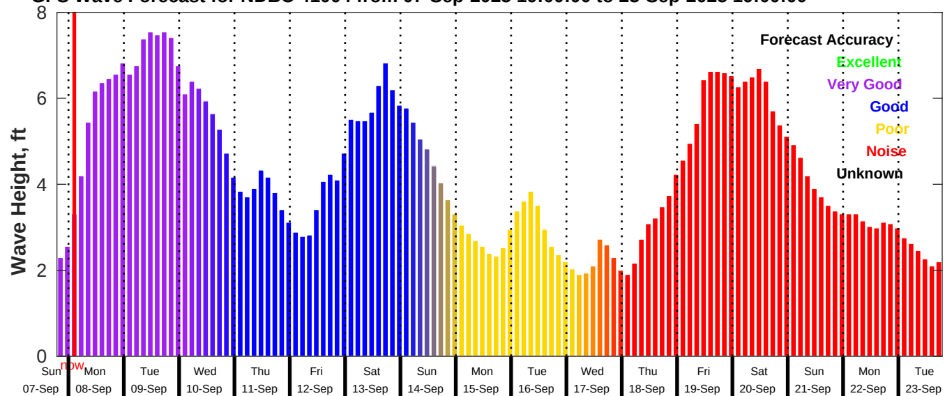
GFS Wave Forecast for NDBC 41004 from 07-Sep-2025 19:00:00 to 23-Sep-2025 19:00:00
