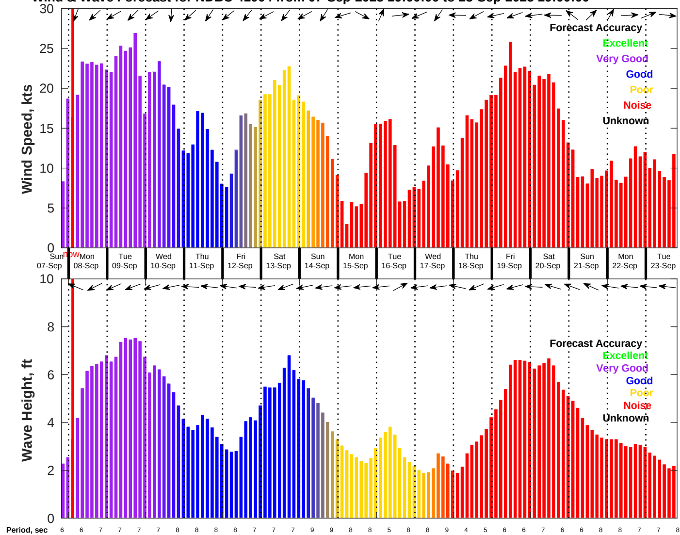
Wind & Wave Forecast for NDBC 41004 from 07-Sep-2025 19:00:00 to 23-Sep-2025 19:00:00
