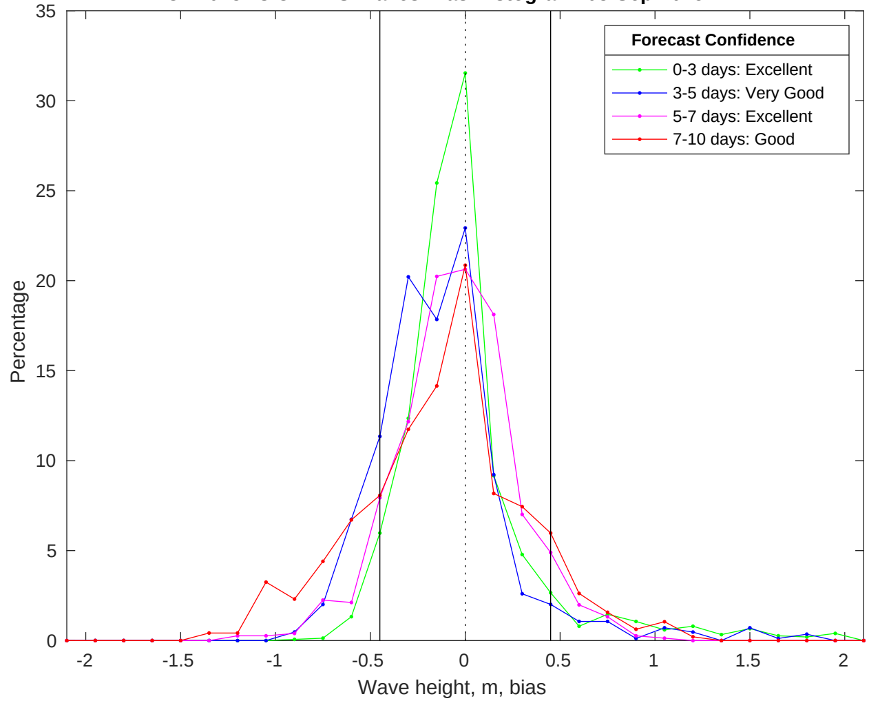
NDBC 41013 vs CMEMS Waves Bias Histogram: 08-Sep-2025
