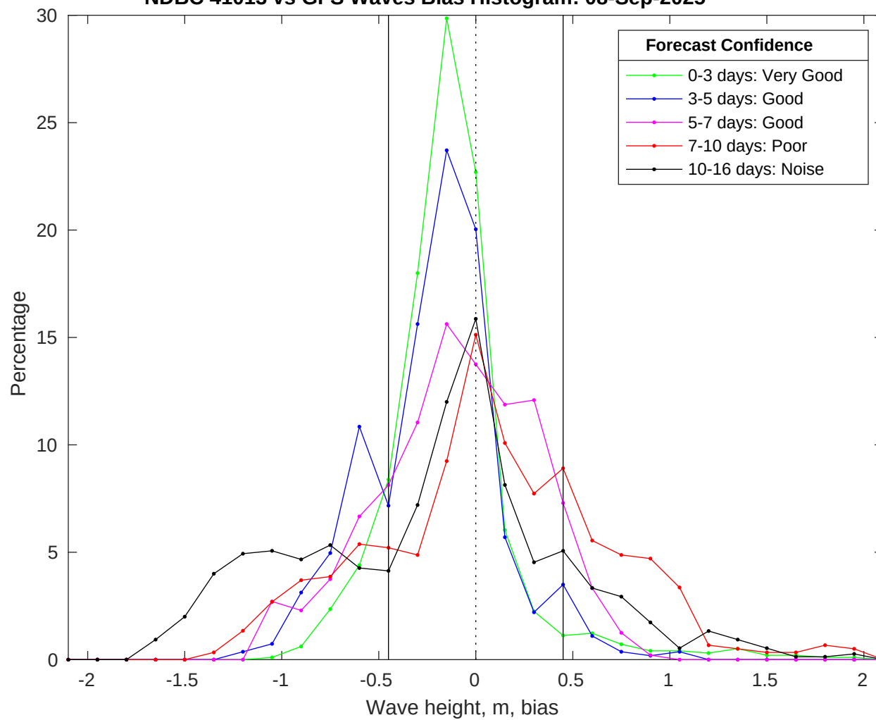
NDBC 41013 vs GFS Waves Bias Histogram: 08-Sep-2025
