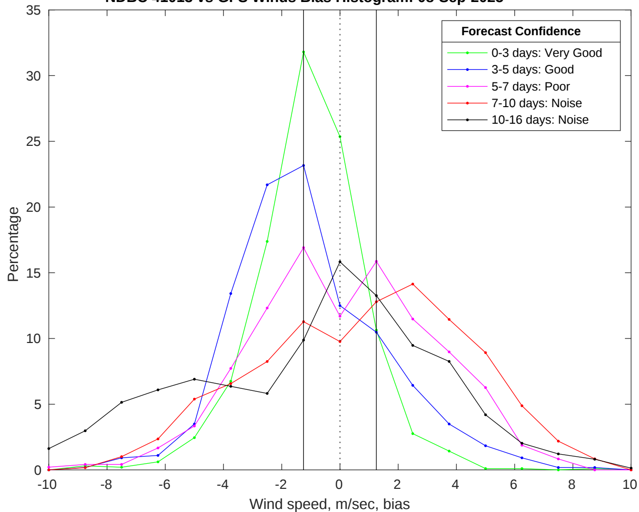
NDBC 41013 vs GFS Winds Bias Histogram: 08-Sep-2025
