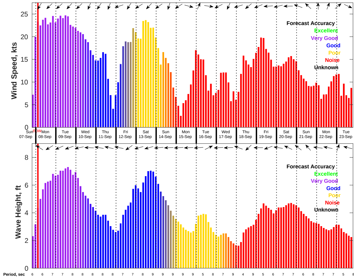
Wind & Wave Forecast for NDBC 41013 from 07-Sep-2025 19:00:00 to 23-Sep-2025 19:00:00
