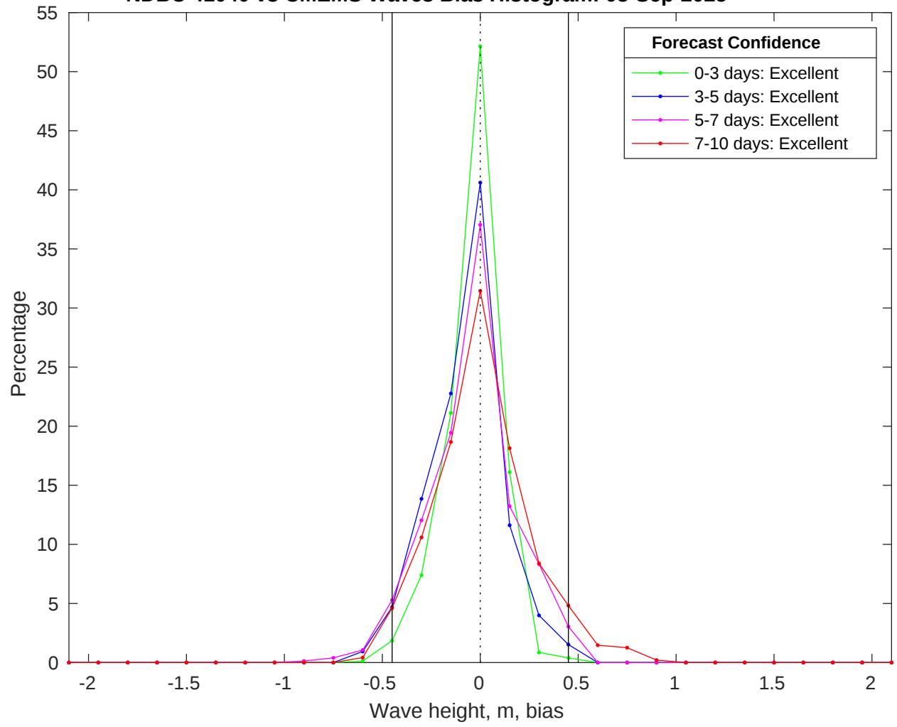
NDBC 41040 vs CMEMS Waves Bias Histogram: 08-Sep-2025
