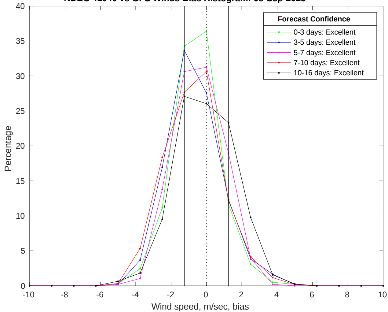
NDBC 41040 vs GFS Winds Bias Histogram: 08-Sep-2025
