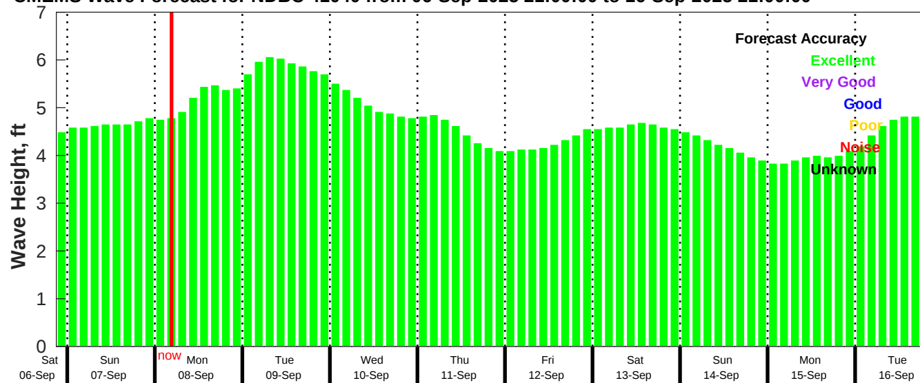
CMEMS Wave Forecast for NDBC 41040 from 06-Sep-2025 21:00:00 to 16-Sep-2025 21:00:00
