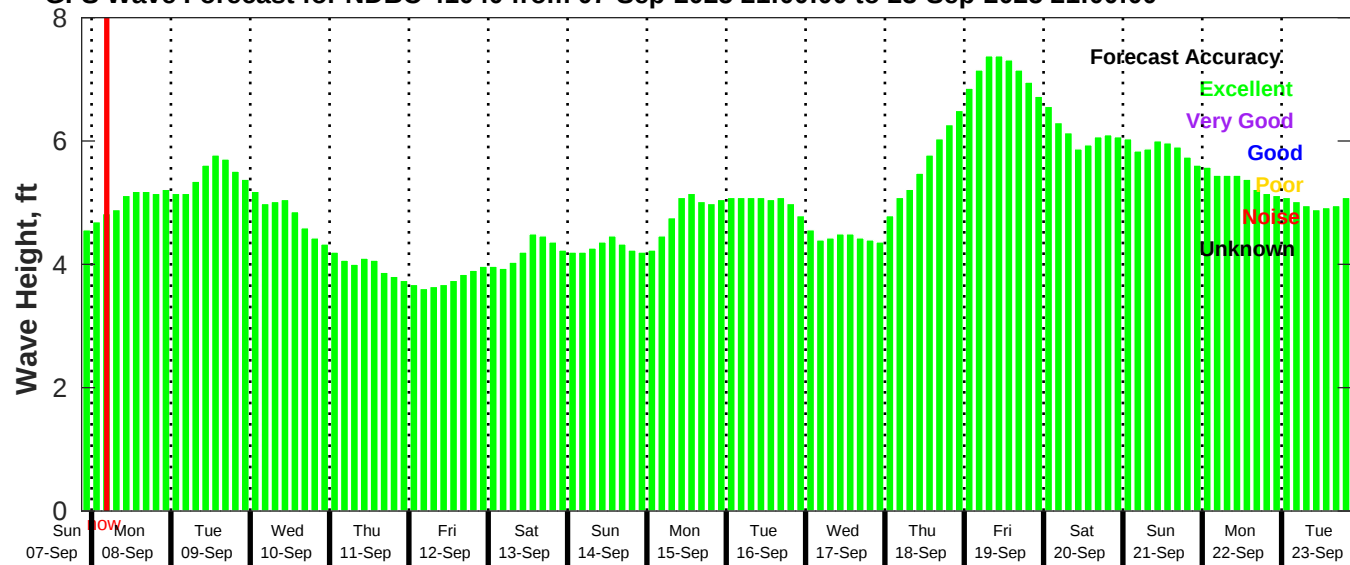
GFS Wave Forecast for NDBC 41040 from 07-Sep-2025 21:00:00 to 23-Sep-2025 21:00:00
