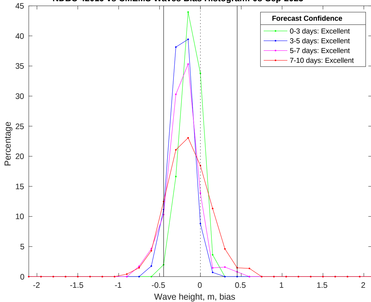
NDBC 42019 vs CMEMS Waves Bias Histogram: 08-Sep-2025
