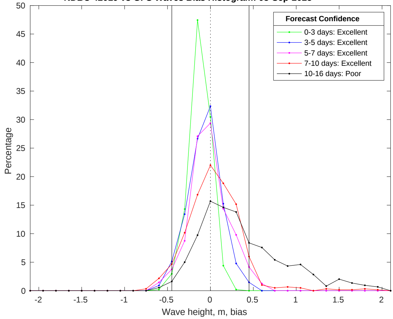
NDBC 42019 vs GFS Waves Bias Histogram: 08-Sep-2025
