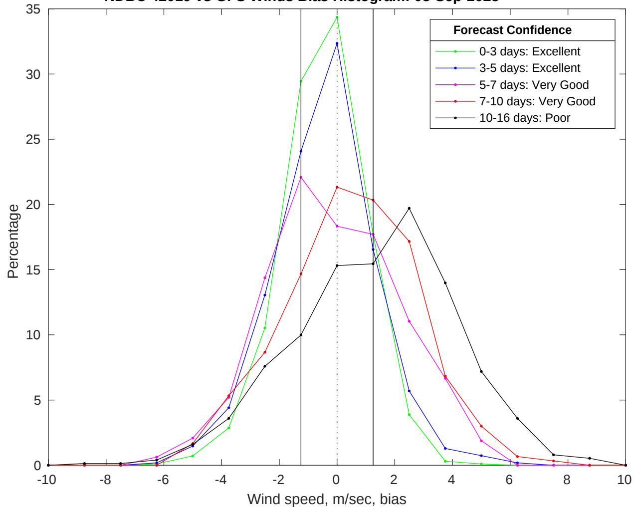
NDBC 42019 vs GFS Winds Bias Histogram: 08-Sep-2025
