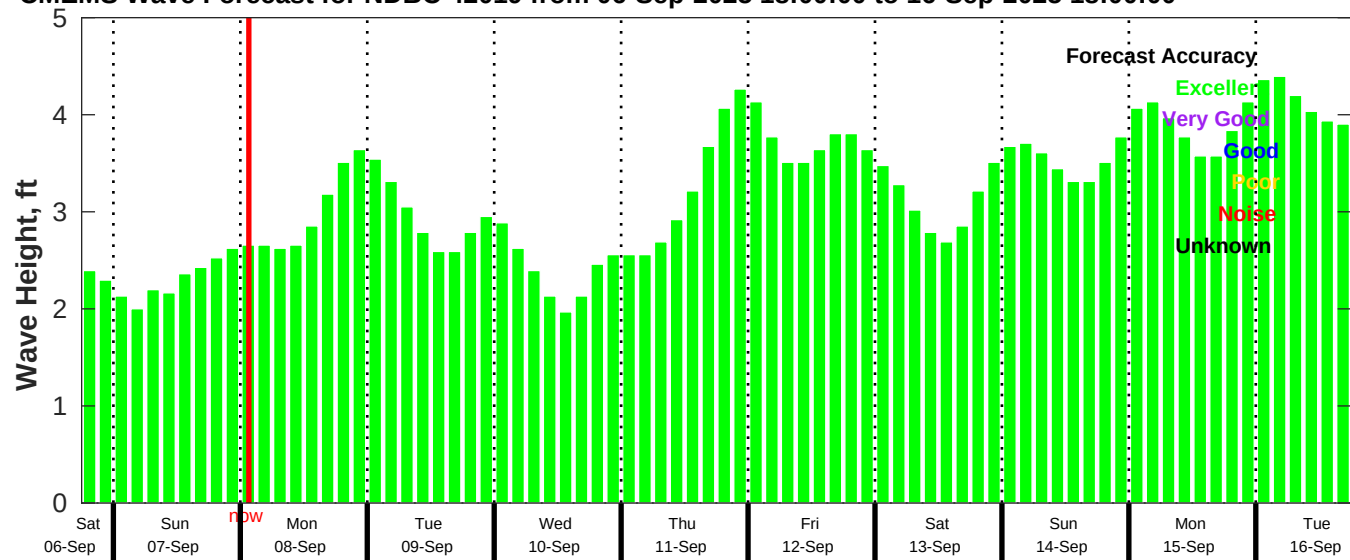
CMEMS Wave Forecast for NDBC 42019 from 06-Sep-2025 18:00:00 to 16-Sep-2025 18:00:00
