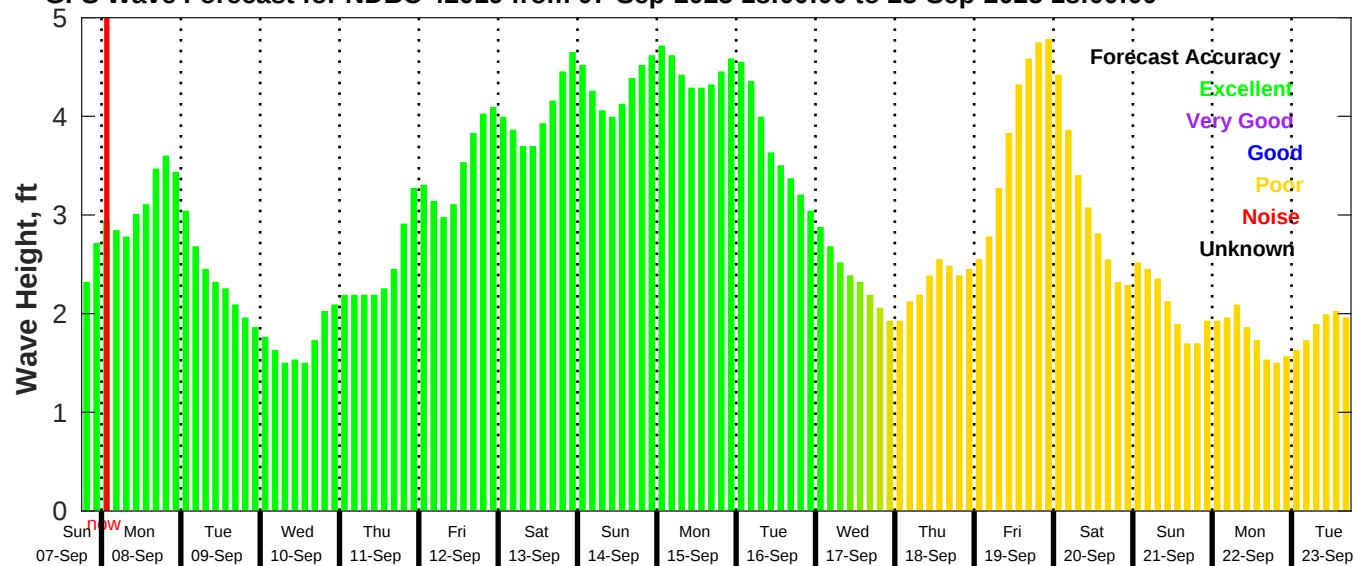
GFS Wave Forecast for NDBC 42019 from 07-Sep-2025 18:00:00 to 23-Sep-2025 18:00:00
