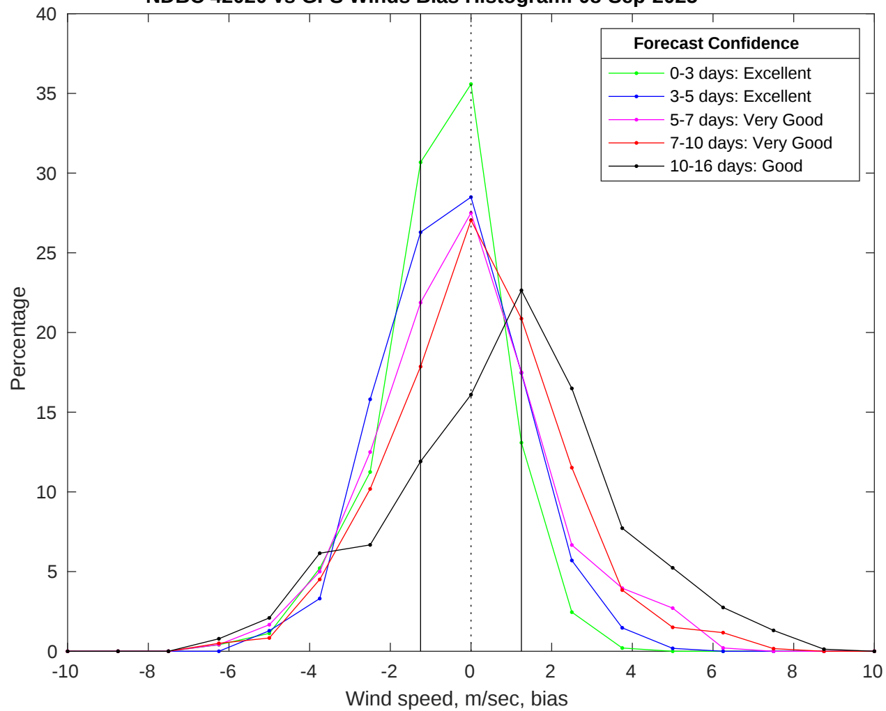
NDBC 42020 vs GFS Winds Bias Histogram: 08-Sep-2025
