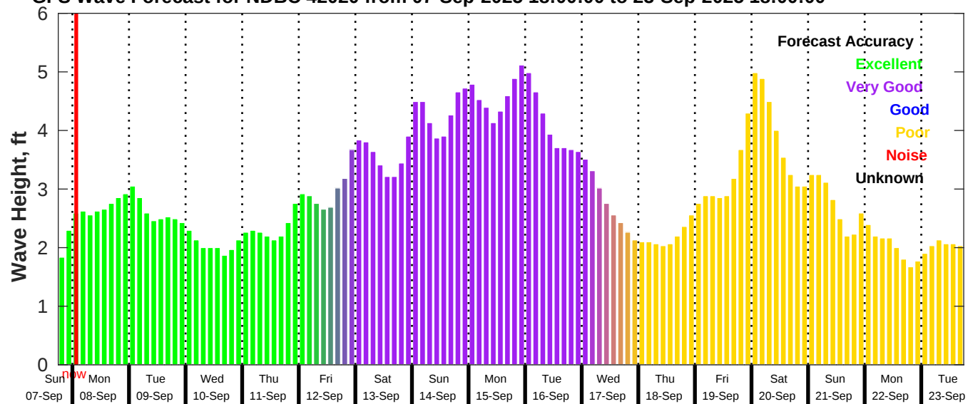
GFS Wave Forecast for NDBC 42020 from 07-Sep-2025 18:00:00 to 23-Sep-2025 18:00:00
