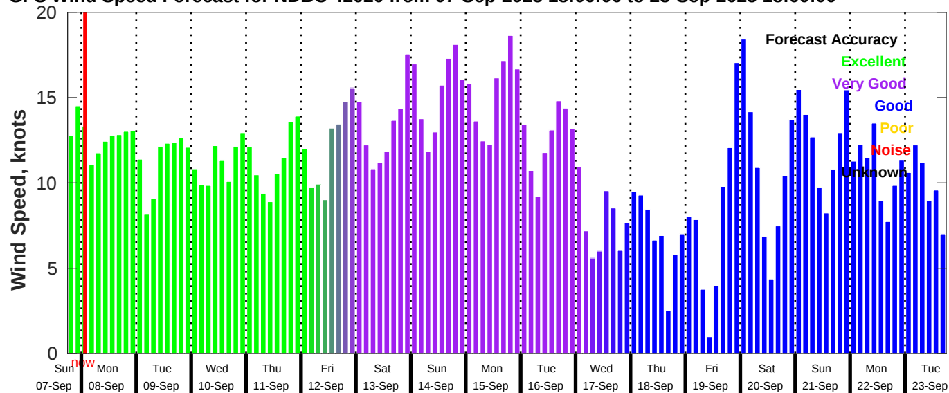
GFS Wind Speed Forecast for NDBC 42020 from 07-Sep-2025 18:00:00 to 23-Sep-2025 18:00:00
