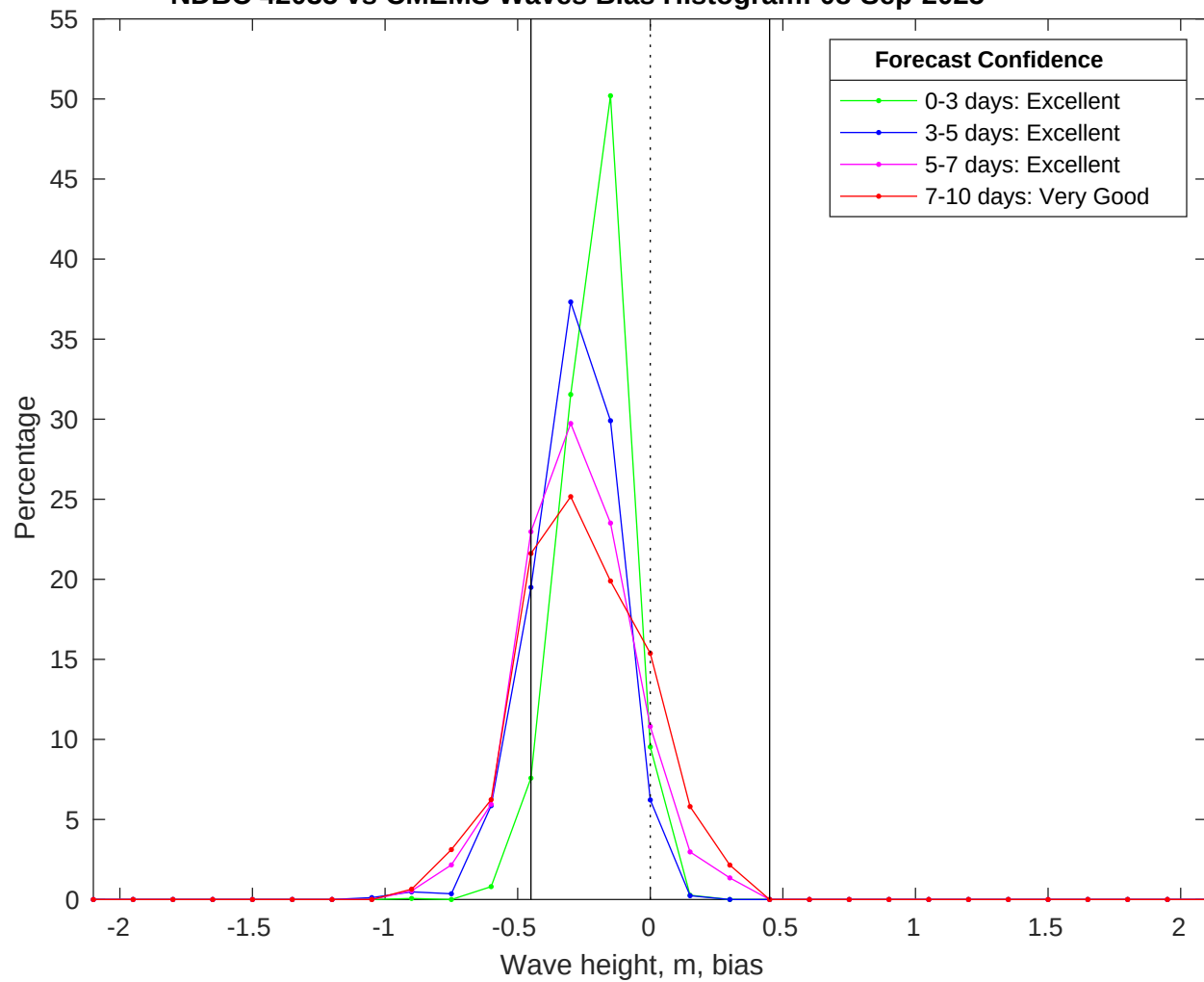
NDBC 42035 vs CMEMS Waves Bias Histogram: 08-Sep-2025
