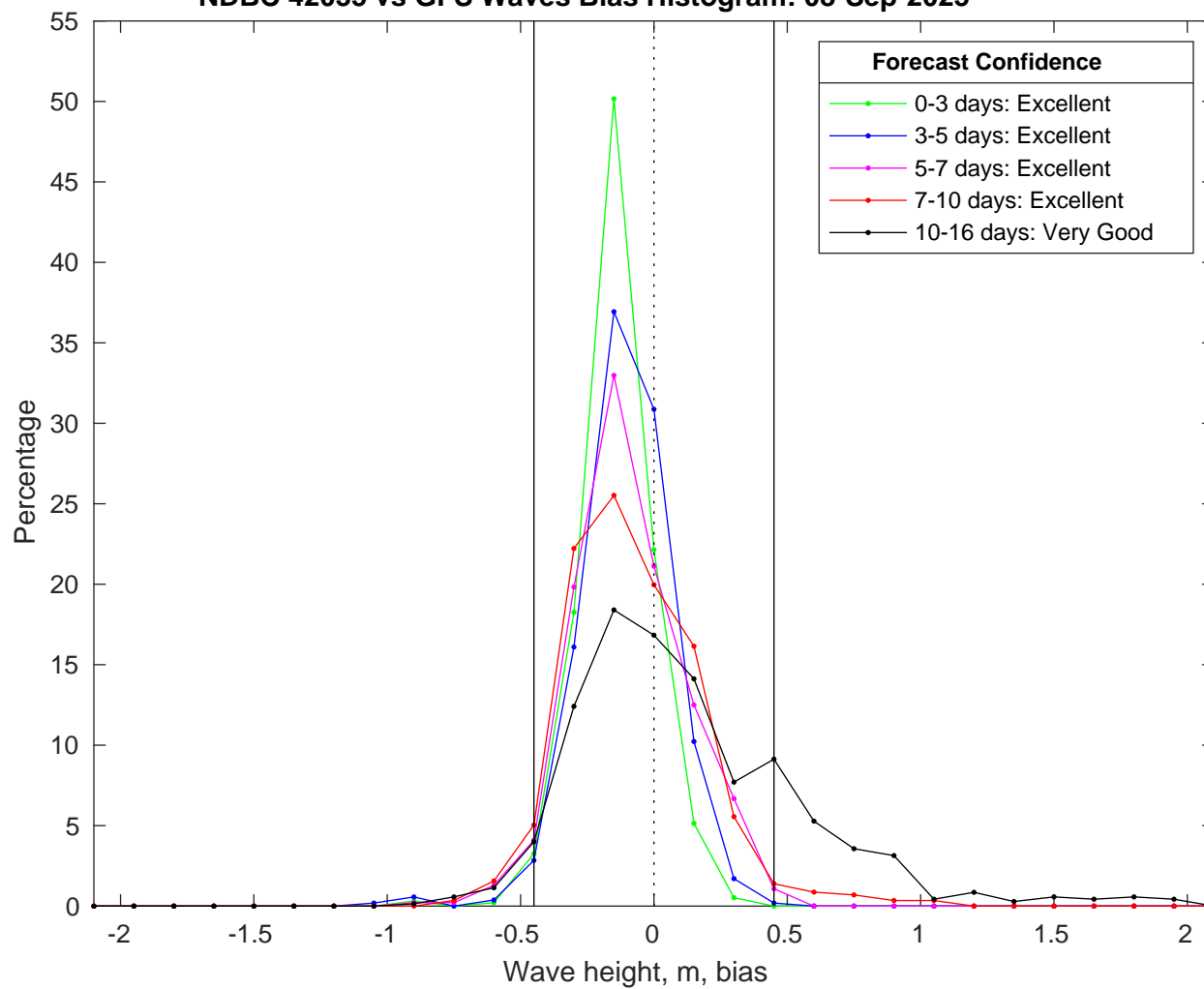
NDBC 42035 vs GFS Waves Bias Histogram: 08-Sep-2025
